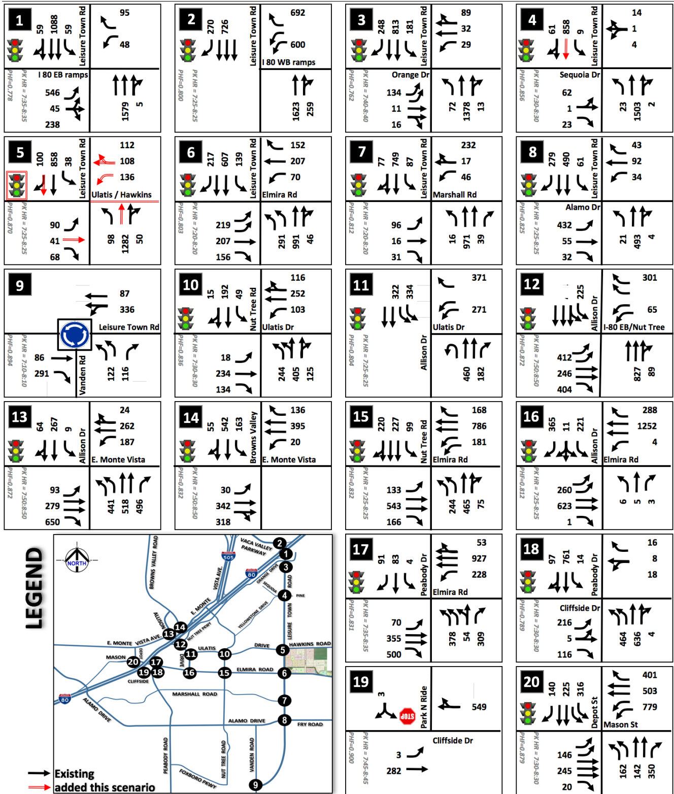
Figure 15. AM Year 2035 Turn Moves, Geometry, and Traffic Control
