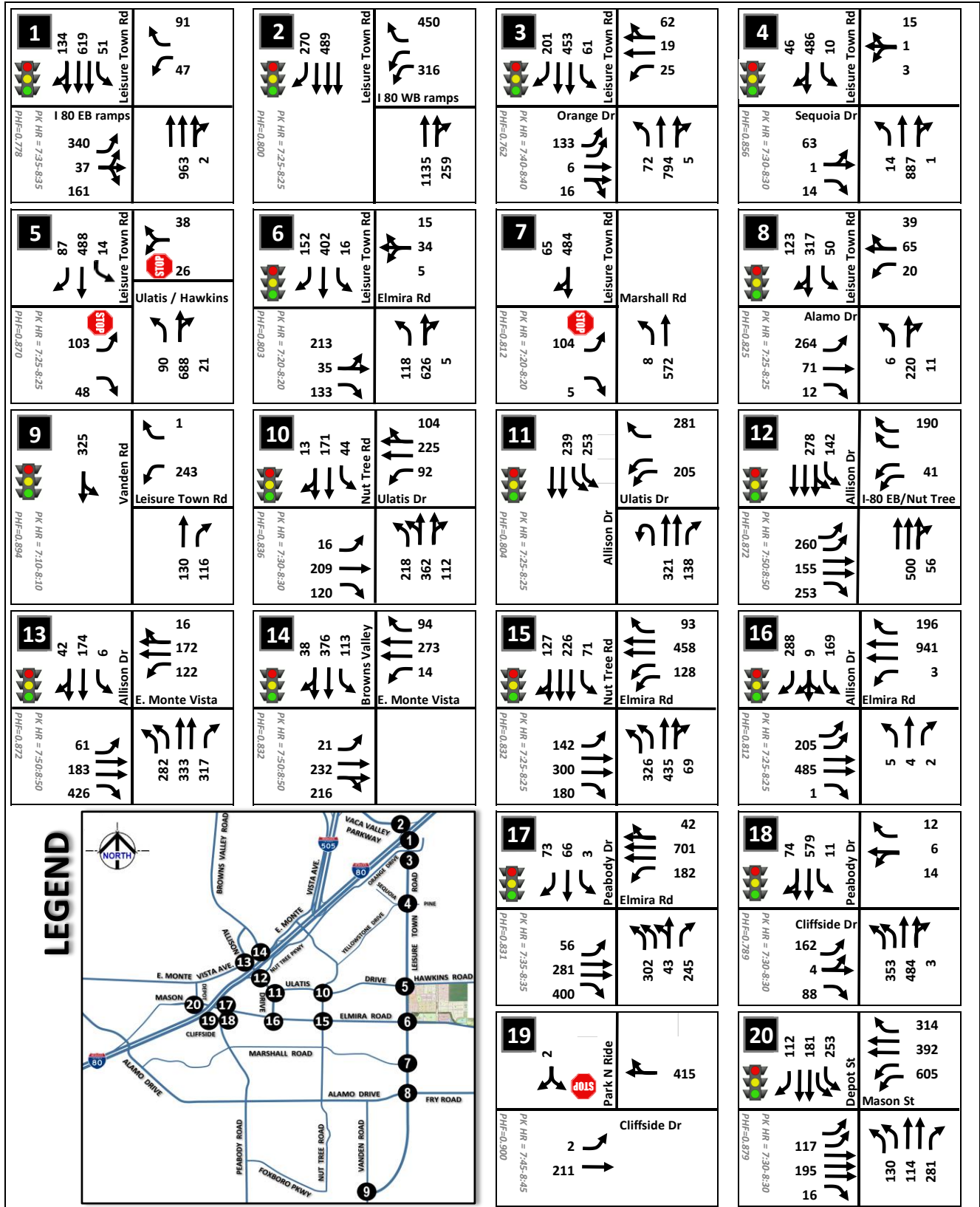
Figure 6. AM Peak Hour Turn Moves, Geometry, and Traffic Control
