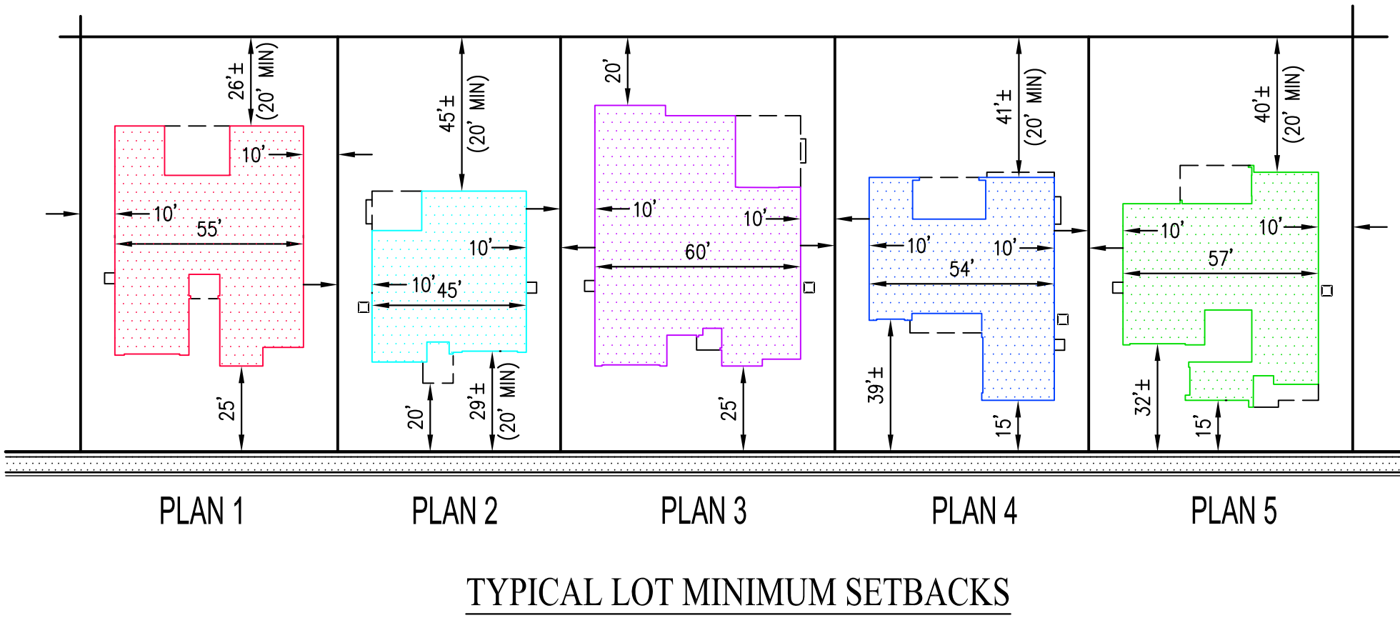
TYPICAL LOT MINIMUM SETBACKS
