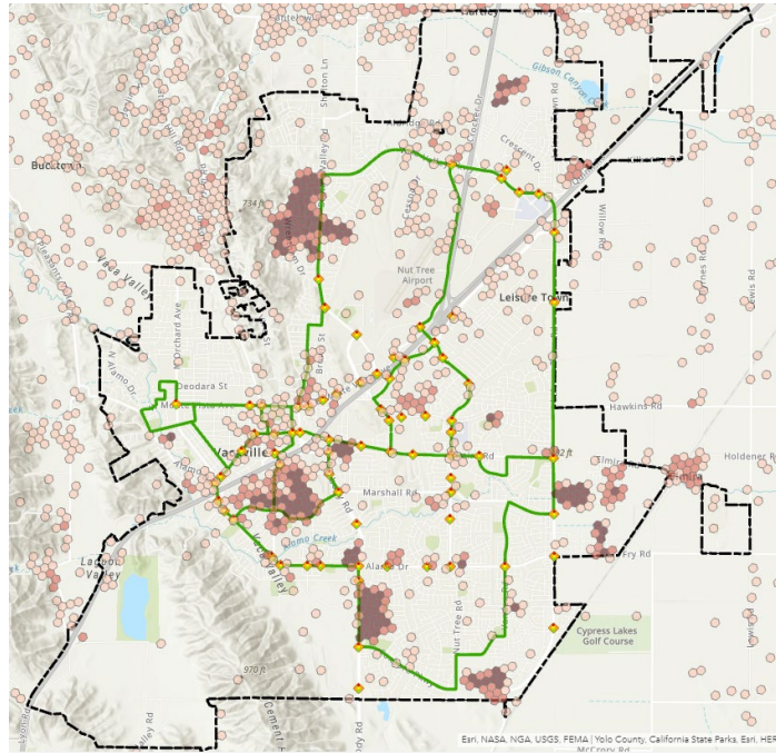
Figure 2 - Phase 1 Unserved Locations & Conceptual Routing
